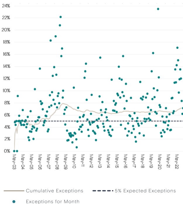
% Exceptions (daily loss > VaR predicted)
