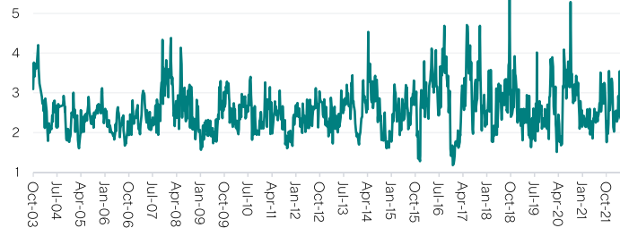
Ratio of Fully Correlated to Regular VaR
